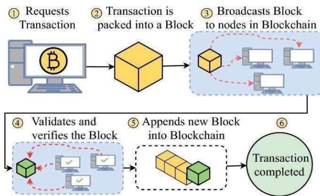
Gambar 2. Proses Blockchain
